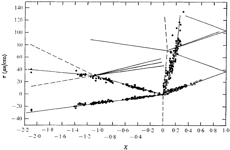
FIGURE 9. \chi , \tau diagram for T_1 = T_0 = 1.46 °K (LHe II). ○, data from the side-mounted liquid detectors; +, apparent arrival of the gas-liquid interface.
